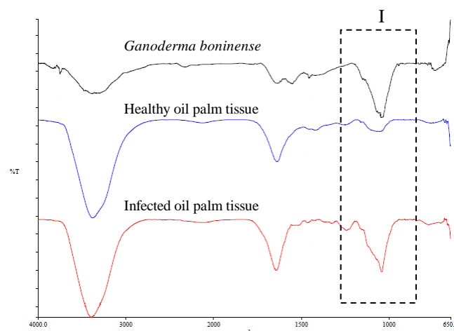
Fig. 1 FTIR spectra of Ganoderma boninense , healthy oil palm trunk tissues and infected oil palm trunk tissues.
