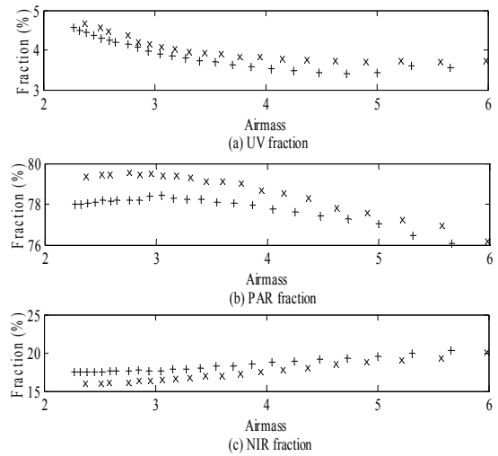
Fig. 5 Diurnal evolution of (a) UV, (b) PAR, and (c) NIR fraction for the two different turbidity days. Symbol + and x represents low and high turbidity day, respectively
