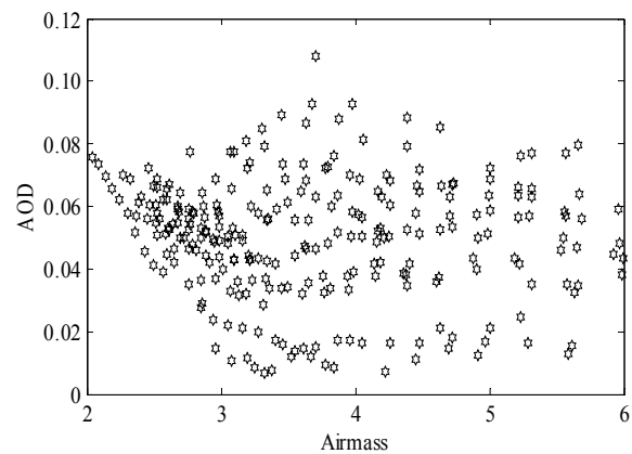
Fig. 3 Variation of AOD at wavelength 550nm for changing air mass during the measurement period
