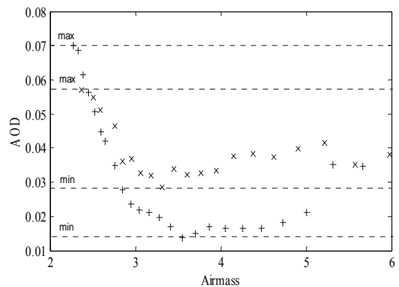
Fig. 6 Diurnal variation of AOD at wavelength 550nm for the two different turbidity days. Symbol + and x represents low and high turbidity day, respectively
